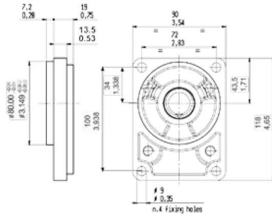
B1 German standard mounting flange
